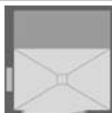
CAB-Q 1400 R.GL * door DIN right / bench seat opposite the door / installation wall left of the door
