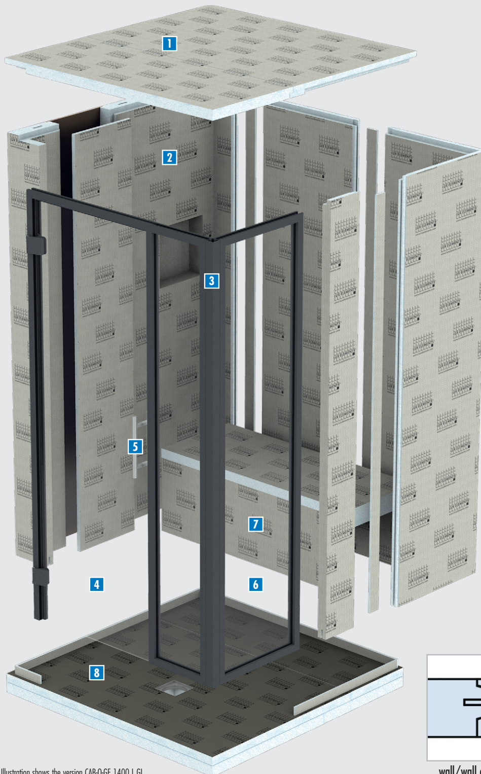
wall/wall connection
