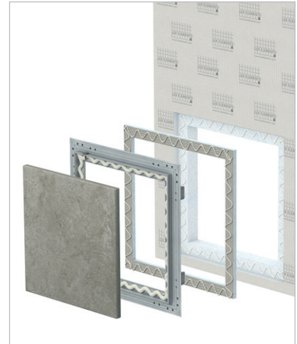
Application with natural stone: without front panel / fillers under frame
